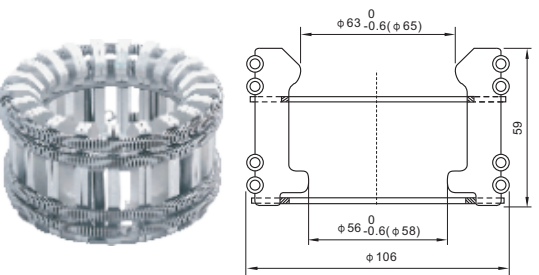
Contact clip: 42 pcs
