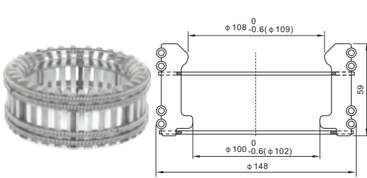
Contact clip: 60 pcs
